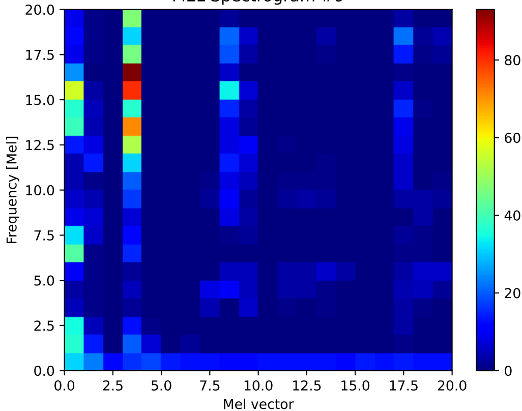
MEL Spectrogram #9
